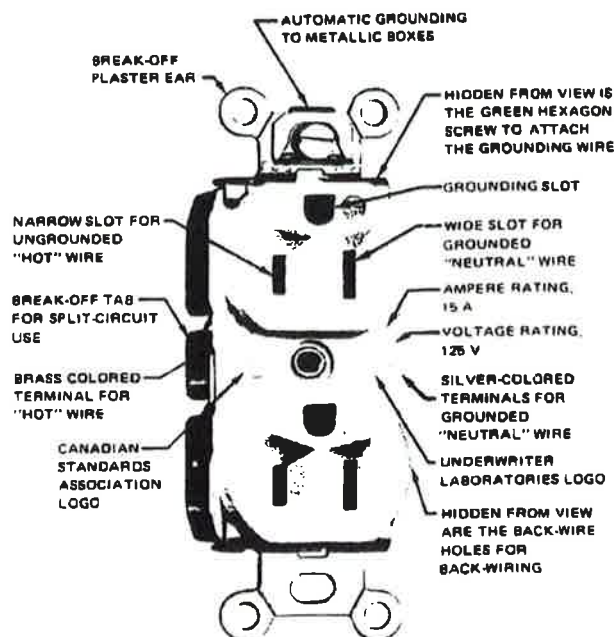
Fig. 5-23 Grounding-type receptacle detailing various parts of the receptacle. Courtesy of Pass & Seymour, Inc.
