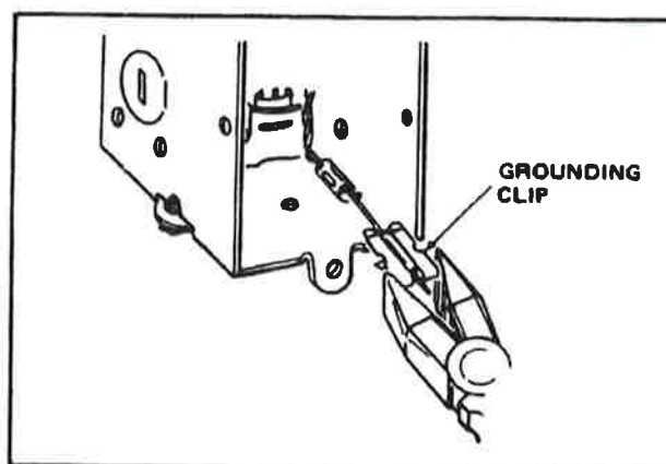
Fig. 5-22 Method of attaching grounding clip to switch (device) box.
