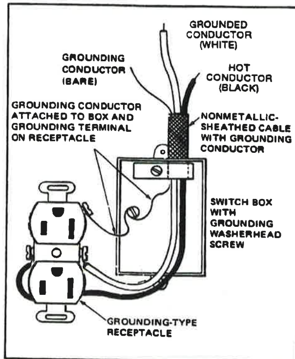
Fig. 5-20 Detail showing connections for grounding-type receptacles.
